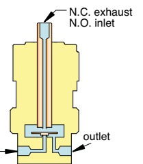
3-Way In-Line Mount
