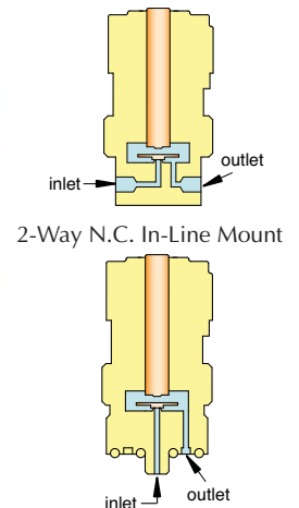
2-Way N.C. Manifold Mount
