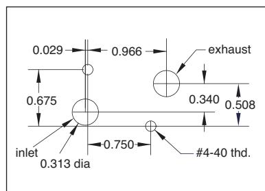
Mounting Interface
