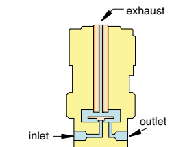
3-Way N.C. In-Line Mount
