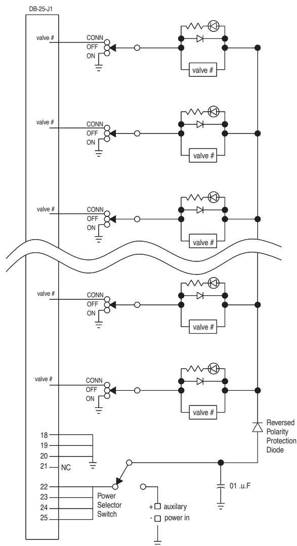
Wiring Diagram
