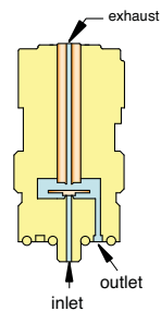
3-Way N.C. Manifold Mount
