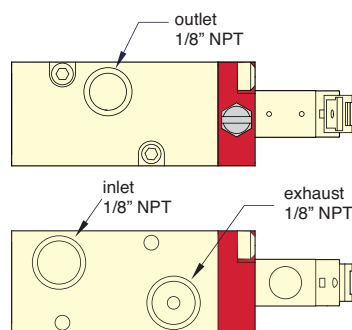
Mounting Interface
