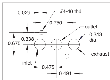
Mounting Interface
